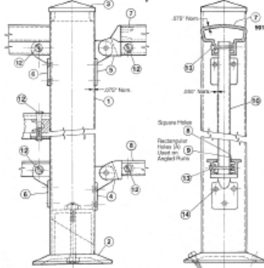
901 Top Rail used with Superior Aluminum Decorative Flat and Corner Columns.
